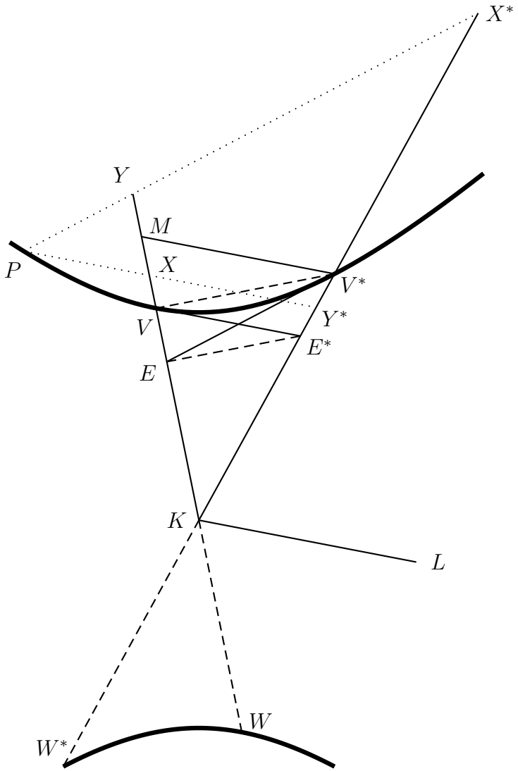
Figure 5: Hyperbola
