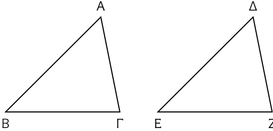
Figure 2.2. Proposition I.4
