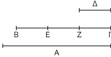
Figure 3.5. Proposition VII.4
